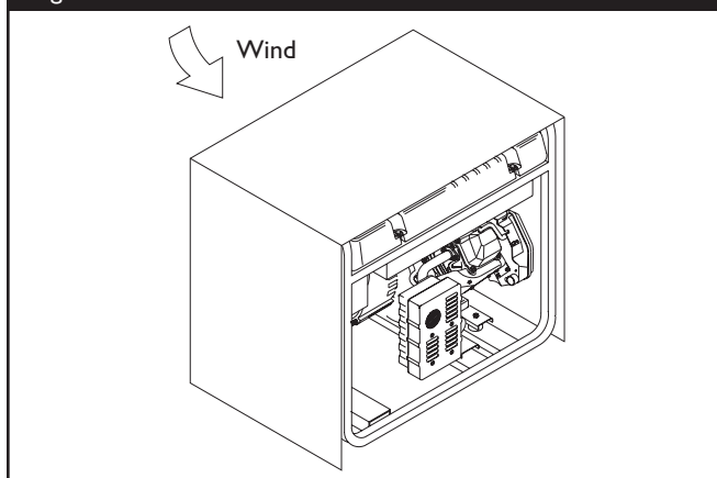
Figure 9 — Permanent Cold Weather Shelter
