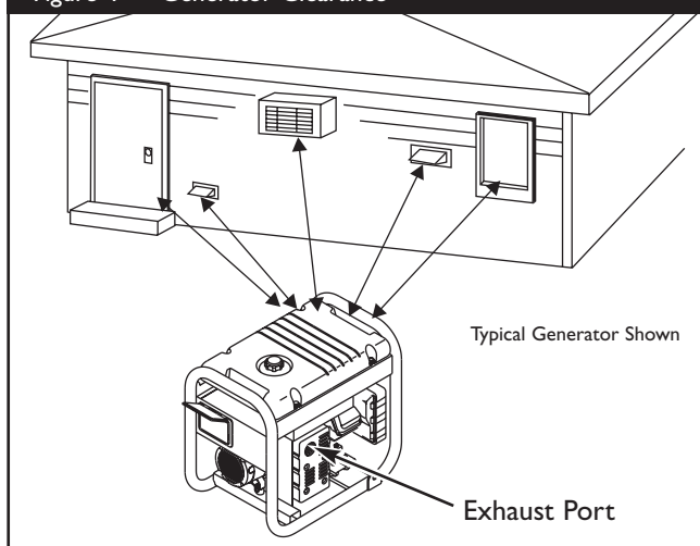
Figure 4 — Generator Clearance
